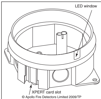
Fig 1 Mounting Box
